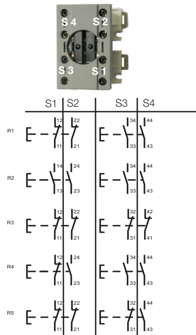
Contact arrangement
