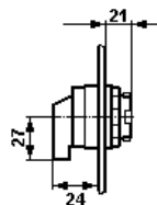
Control switch
